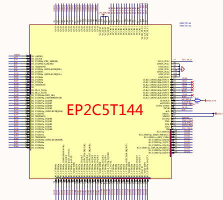
EP2C5T144C8N
